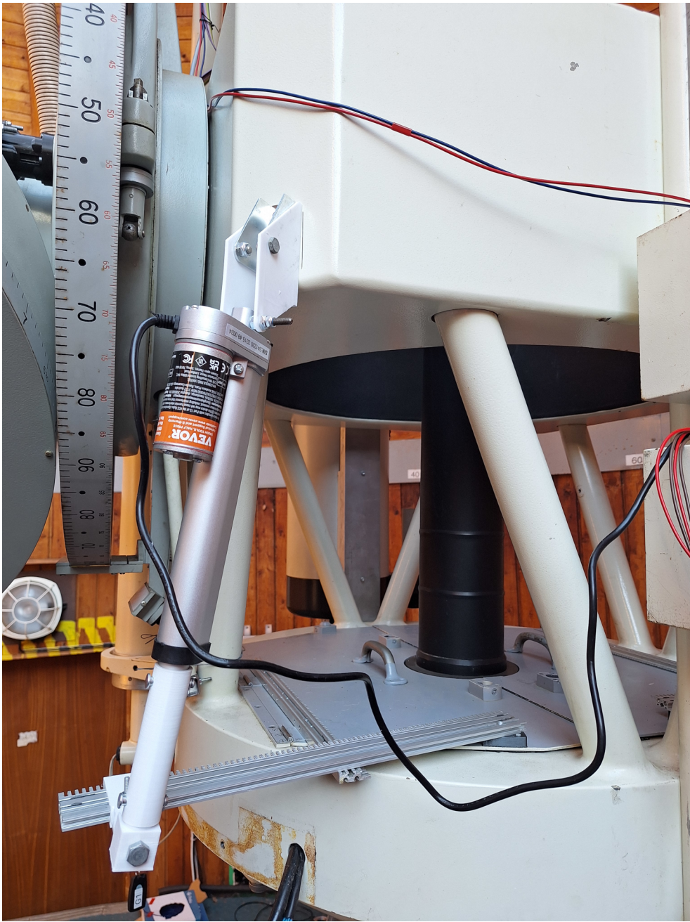
Linear actuators, scrapy aluminium extrusions and some 3D printed parts
