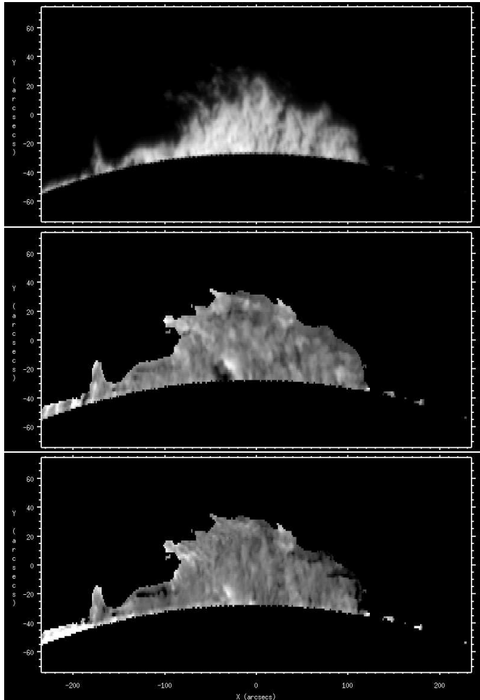
Figure 1. The line profile amplitude (top panel), the Doppler velocity (middle panel), and the Gaussian line width (bottom panel) of the H\alpha spectral line derived for the quiescent prominence observed on 20/10/2012 at 07:06 UT at the position angle 170^\circ . The displayed ranges are \pm 12 km/s for the Doppler shift range and 0.020-0.045 nm in case of the Gaussian line width.
