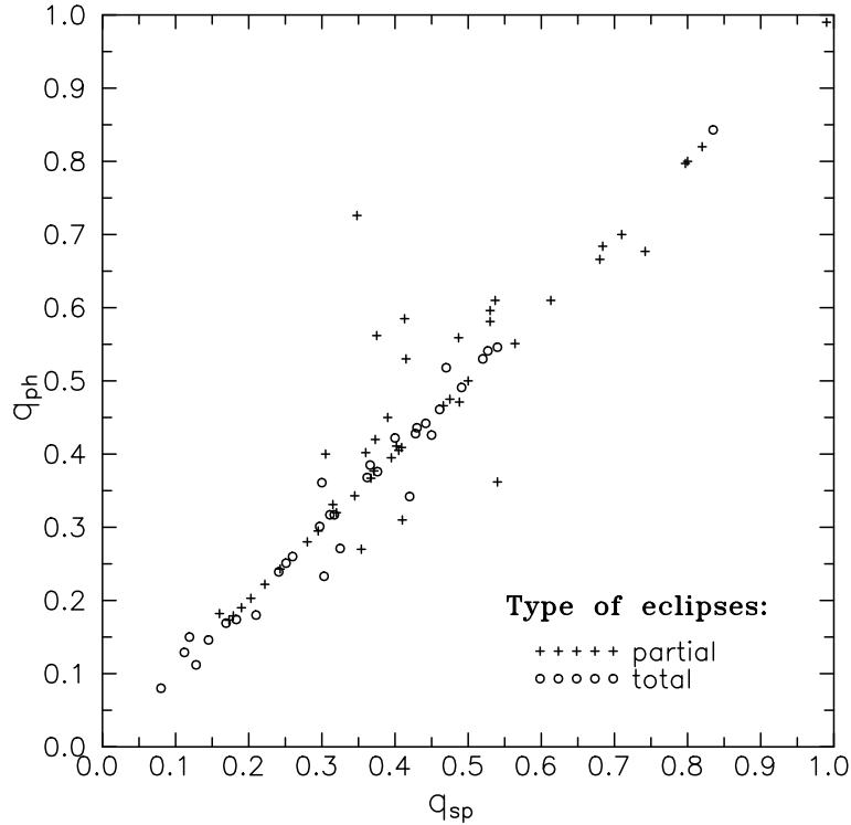
Figure 1. Spectroscopic versus photometric mass ratios for contact binaries in the first group with known type of eclipses (total/partial)
