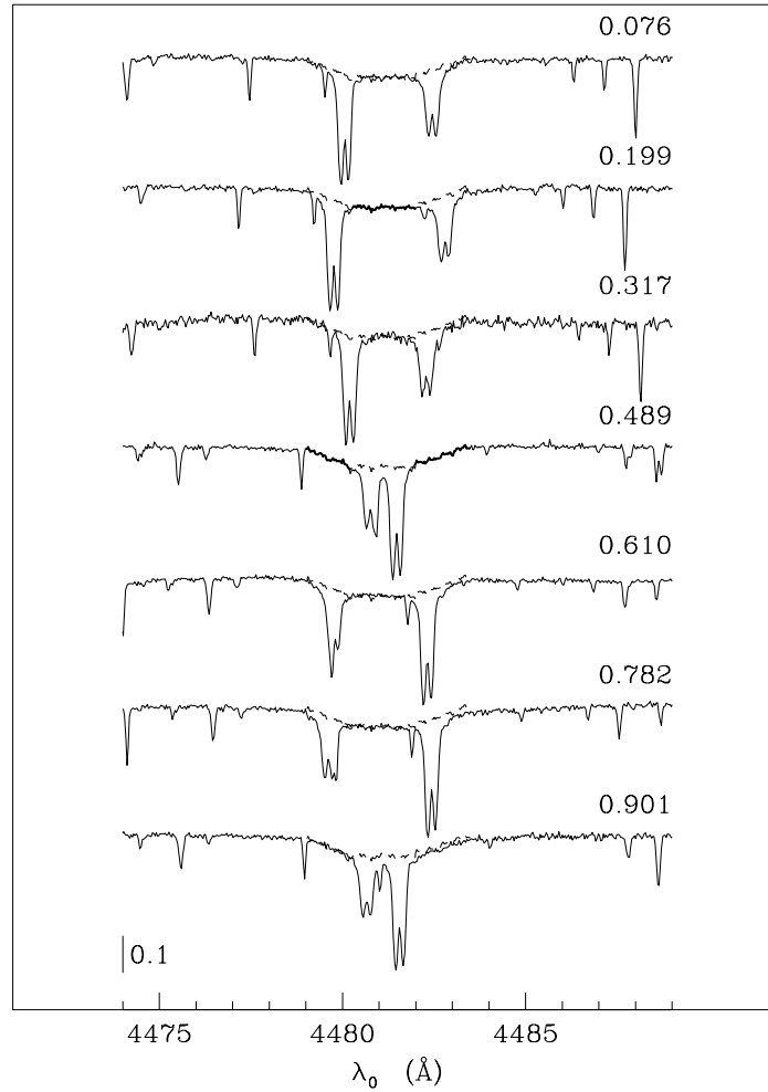
Figure 1. The triple system 74 Aqr at various orbital phases
