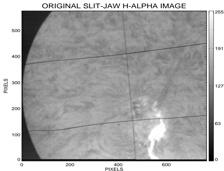
Figure 1: The full field of view of the slit-jaw system of the Vacuum Tower Telescope in H \alpha . The vertical line is the slit, the two horizontal wires are used to mark the area of spectral investigations. The color bar units are expressed in Arbitrary Intensity Units (AIU).
