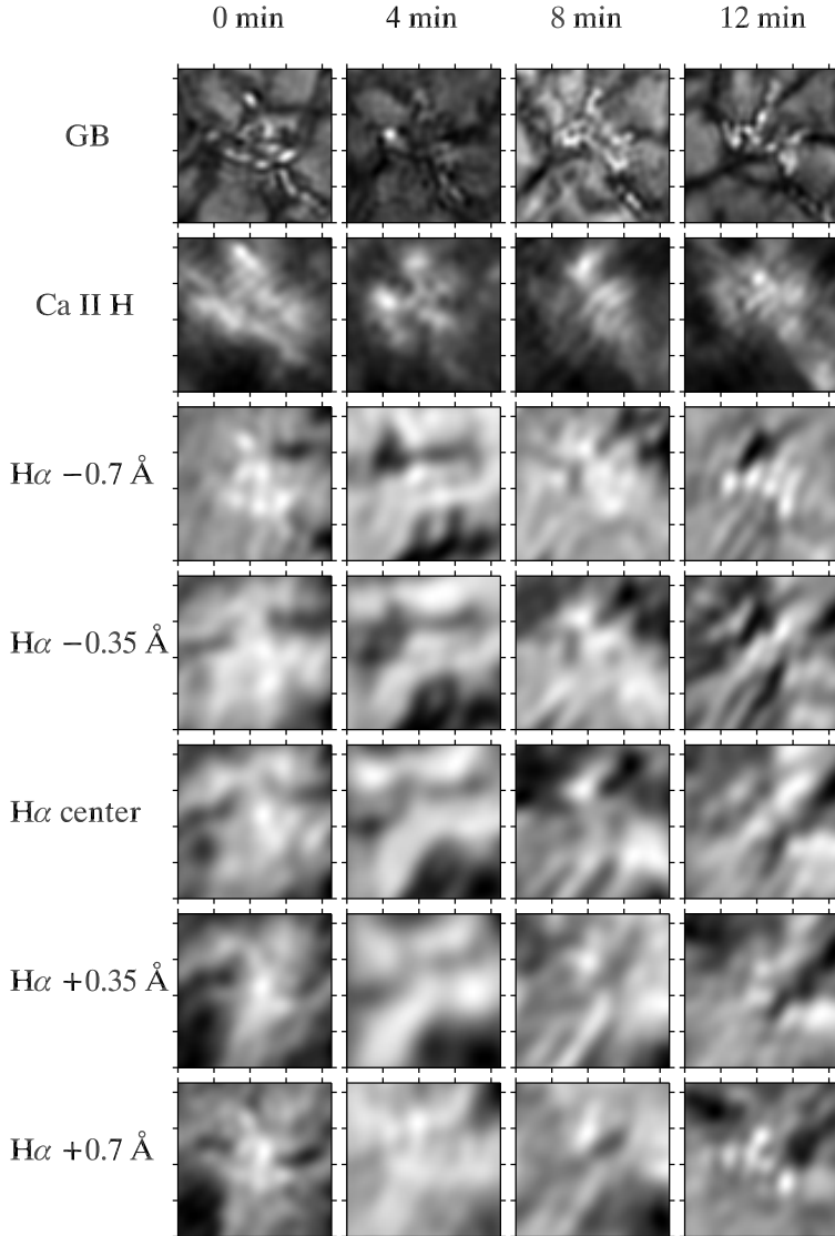
Figure 4. Temporal evolution of the selected network element seen simultaneously in the DOT G-band, Ca II H, and H\alpha images taken at five wavelength settings of the H\alpha Lyot filter. The time 0 min corresponds to the moment of the start of the observation at 09:55:20 UT. Field of view: 4.3 \times 4.3 \text{ arcsec}^2 . Tickmark spacing: 1 arcsec.
