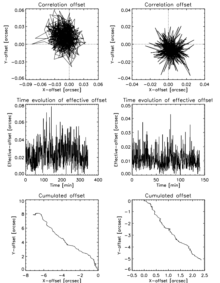
Fig. 1. Hinode/SOT pointing stability for data sets I (left) and II (right). Top row: the displacement between an image and the succeeding one ( \Delta y versus \Delta x ). The dotted lines indicate stable satellite pointing. It can be seen that the actual barycenter of the displacements is shifted diagonally out of this point (drift). Middle row: effective ( \sqrt{\Delta x^2 + \Delta y^2} ) displacements versus time. Bottom row: cumulated displacements in x - and y -direction, which reflects the satellite pointing on the solar surface.
