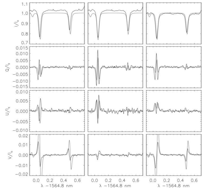
Fig. 13. Comparison of observed ( black ) and synthetic spectra ( gray ) in step 4. Top to bottom: Stokes IQUV . Left to right: Lower footpoint, center of loop, upper footpoint.
