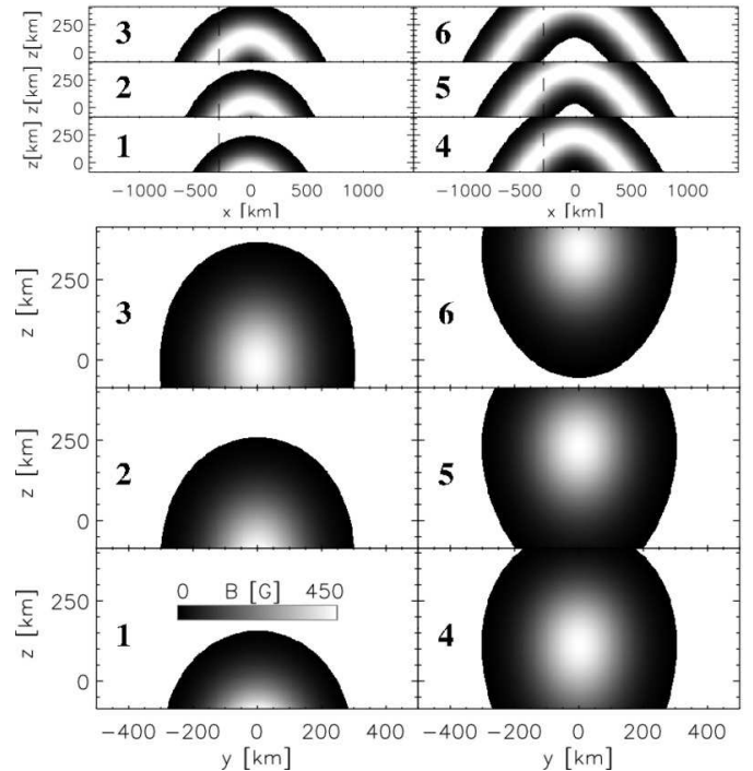
Fig. 10. Magnetic field strength in side view in the x - z plane ( top ), and cut in the y - z plane across one of the footpoints ( bottom ). The location of the cut is marked by a dash-dotted vertical line in the upper plot.
