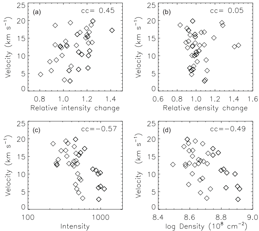
Figure 5. Correlation plots of the EIS Fe XIII LOS velocity against the relative changes (top) and absolute values (bottom) of the intensity and density at the EIT wave front.
