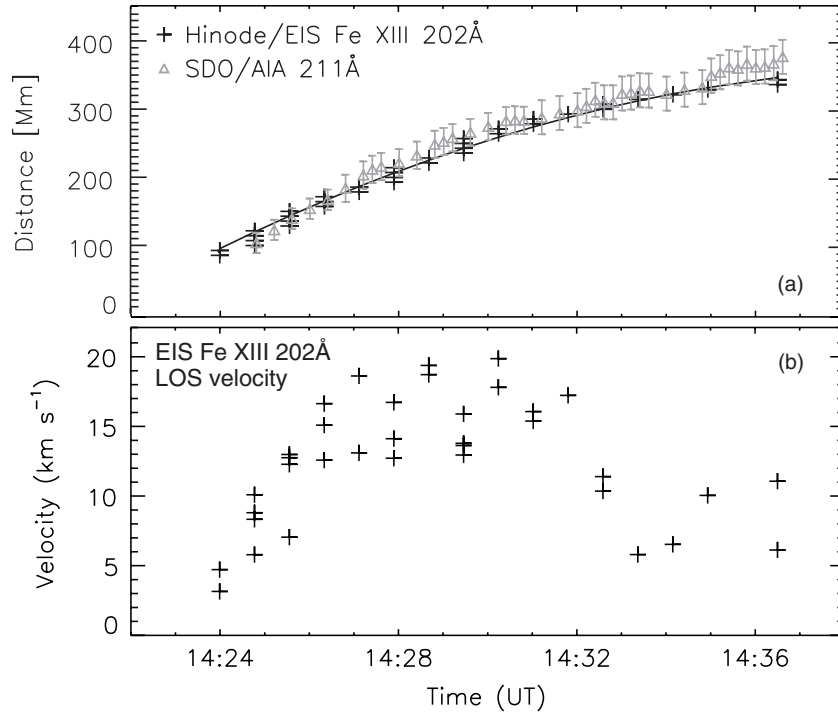
Figure 4. (a) Kinematics of the EIT wave derived from the EIS Fe XIII LOS velocity peaks (crosses) and from the wave fronts identified in SDO/AIA 211 Å images (triangle with error bars). (b) Evolution of the EIS Fe XIII LOS velocity peaks derived at the EIT wave front (cf. Figure 3, bottom).
