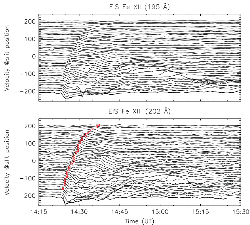
Figure 3. Velocity profiles derived from the EIS Fe XII (top) and Fe XIII (bottom) spectrograms (only each 10th profile available is plotted). Each profile starts at the y-position along the slit. The circles plotted on top of the Fe XIII profiles indicate the position of the peak LOS velocity at the wave front. These positions/values are used for the EIS wave kinematics (Figure 4(a)) and LOS velocity evolution (Figure 4(b)) as well as for the correlation plots in Figure 5.
