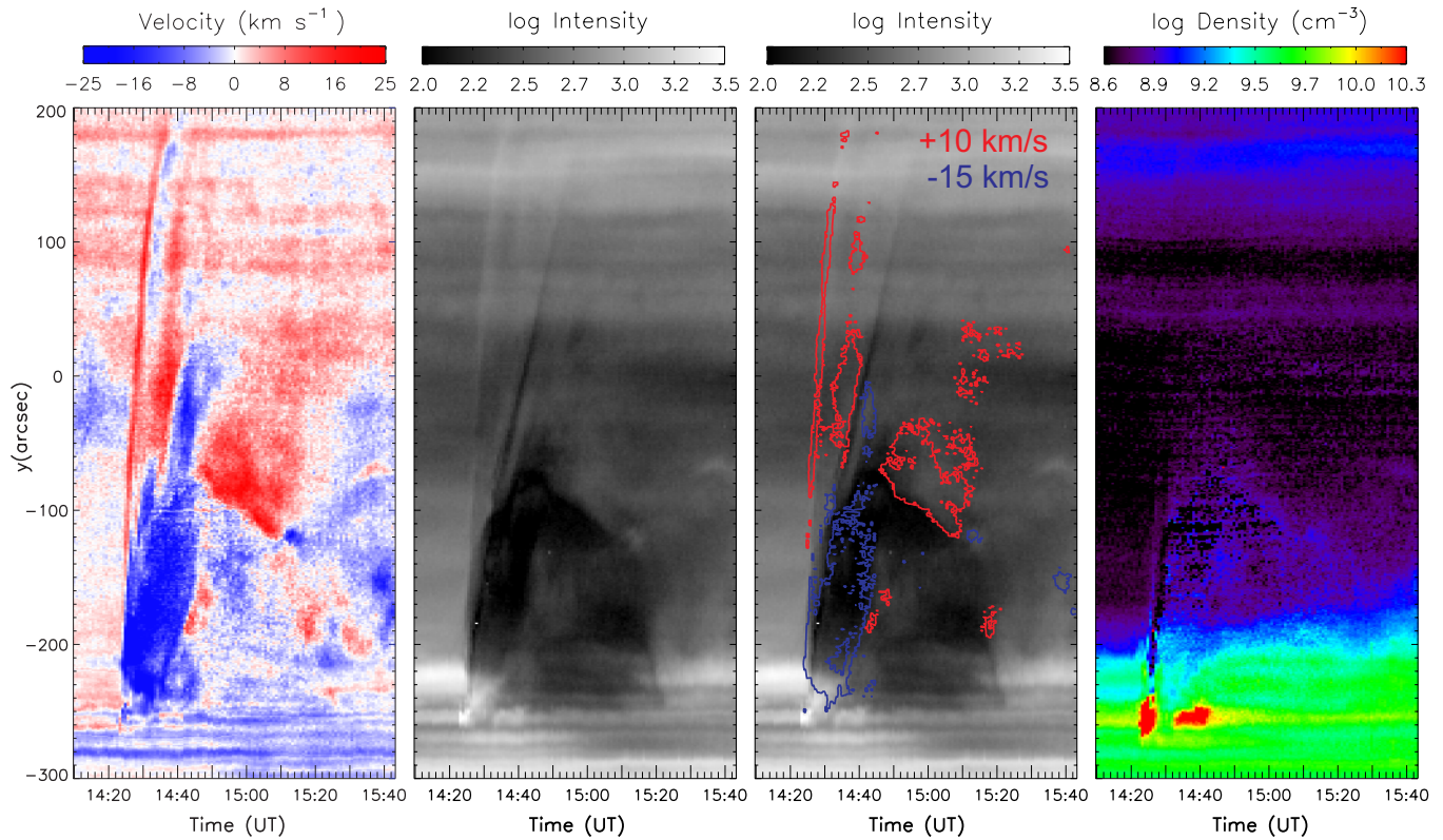
Figure 2. Stack plots showing the Fe XIII 202 Å evolution along the EIS slit during the time range 14:10 to 15:42 UT: (a) velocities, (b) intensities, (c) intensities together with velocity contours at -15 \text{ km s}^{-1} (blue) and +10 \text{ km s}^{-1} (red), and (d) densities derived from the Fe XIII 202/203 Å line pair.
