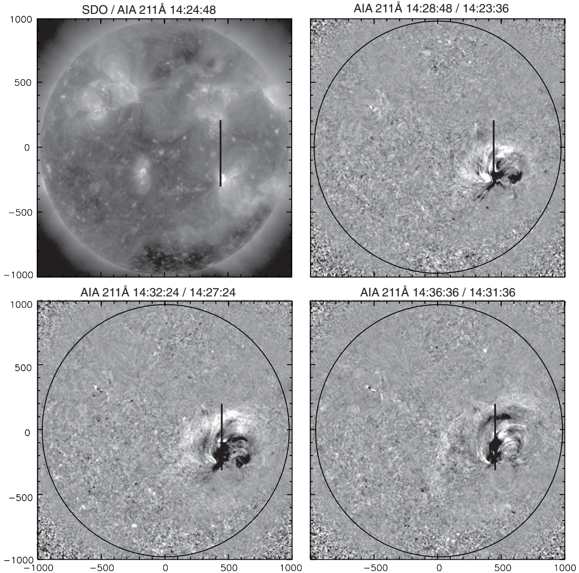
Figure 1. Sequence of SDO /AIA 211 Å direct (top left) and running ratio images. The vertical line indicates the position of the Hinode /EIS spectrometer slit. The accompanying movie 1 shows the EIT wave evolution in SDO /AIA 211 Å direct and running ratio images. Movie 2 shows the same in the SDO /AIA 193 Å filter.
